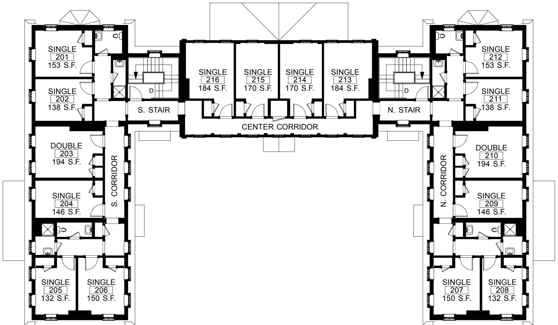
Triangle House - 2nd Floor Plan
